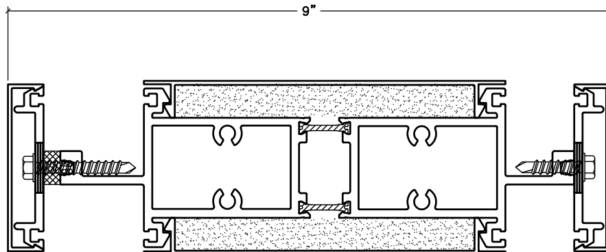
CURTAINWALL FRAME
