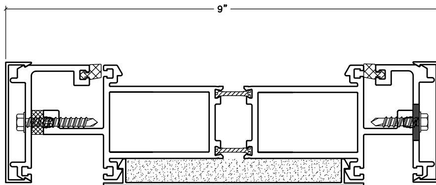
CURTAINWALL FRAME
