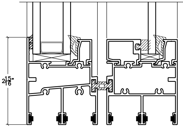
TRIPLE GLAZE
