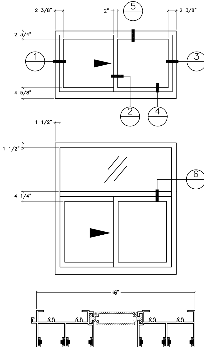
VENETIAN BLIND FRAME
