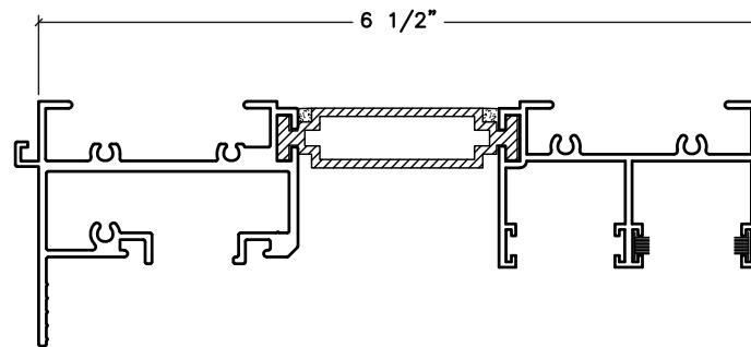
VENETIAN BLIND FRAME
