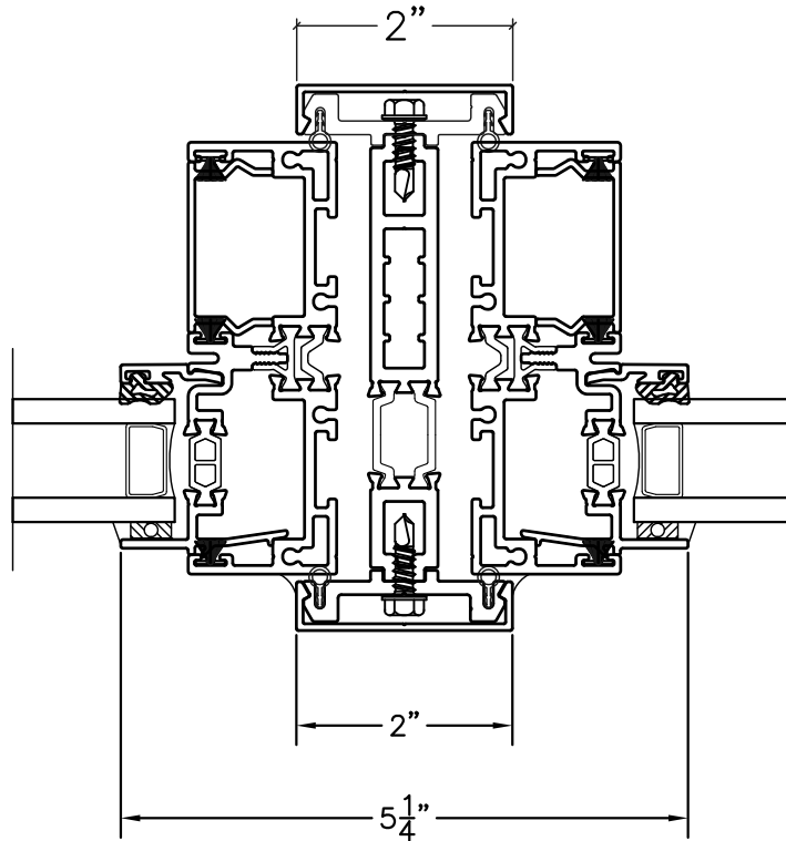
5-PIECE MULLION HORIZONTAL OR VERTICAL
