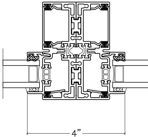
H-BAR MULLION HORIZONTAL OR VERTICAL
