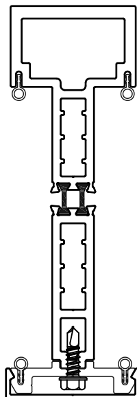
HEAVY 3-PIECE MULLION HORIZONTAL OR VERTICAL
