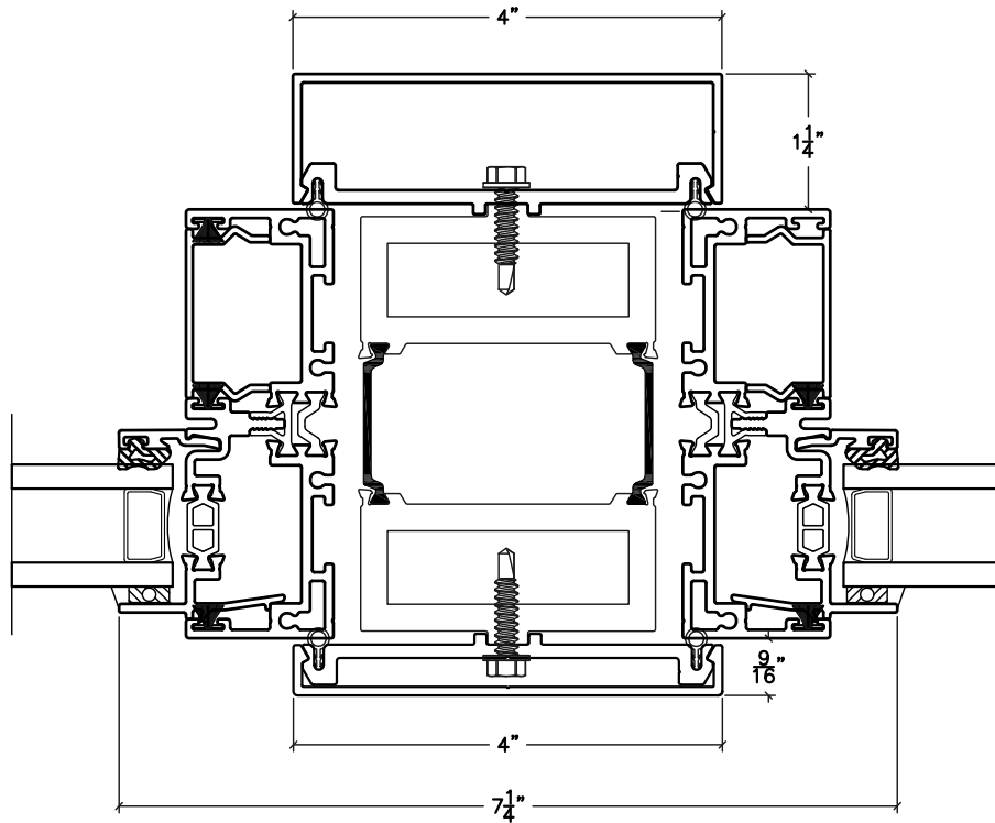
STRUCTURAL 5-PIECE MULLION HORIZONTAL OR VERTICAL
