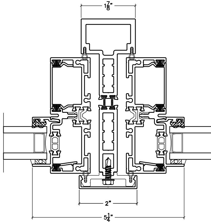
HEAVY 3-PIECE MULLION HORIZONTAL OR VERTICAL
