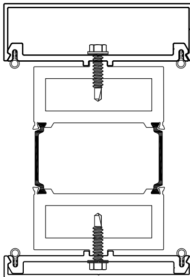
STRUCTURAL 5-PIECE MULLION HORIZONTAL OR VERTICAL
