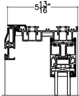
5000 SLIDING
