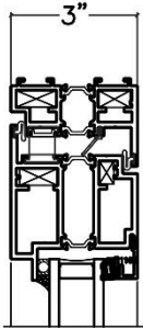
3000 TERRACE
